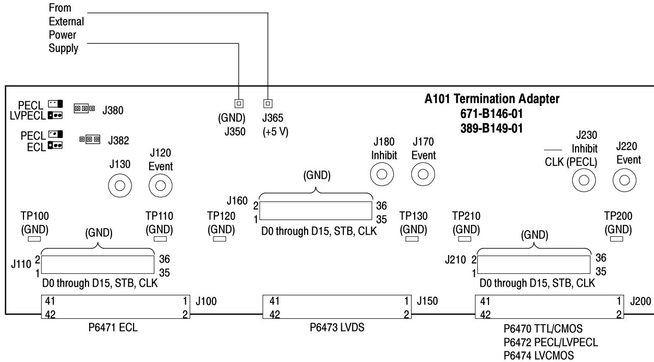
Figure 4-1: Termination Board
